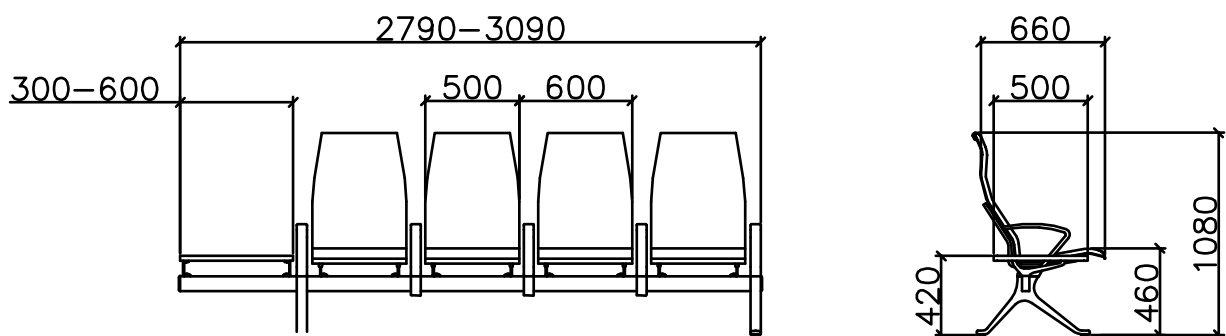
FLY II STAINLESS STEEL HIGHBACK - 4-SEATER + TABLE - TECHNICAL DRAWING
