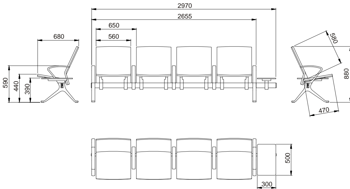
FLY II PU - 4-SEATER + TABLE - TECHNICAL DRAWING
